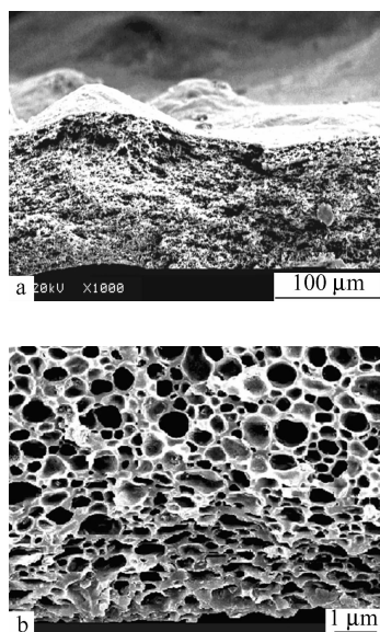
Fig. 8 SEM photographs of the cross-section of TSPU membrane at 20°C
