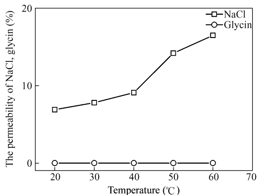
Fig. 11 The permeability of NaCl and glycine (in 1 h) as a function of temperature
