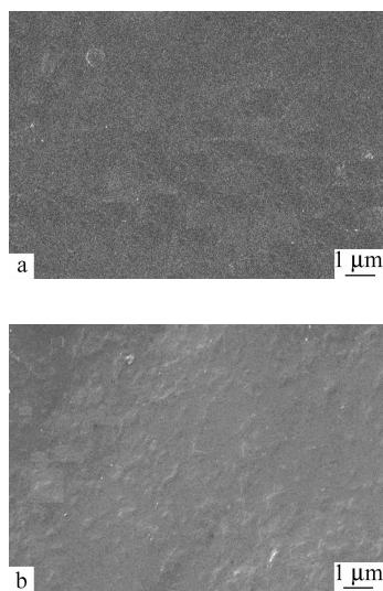
Fig. 6 SEM photographs of the top (a) and bottom surface (b) of TSPU membrane at 20 °C
