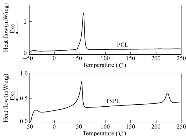
Fig. 3 DSC curves of PCL and TSPU
