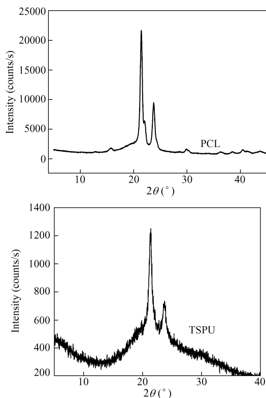
Fig. 4 XRD graphs of PCL and TSPU membrane at 25°C
