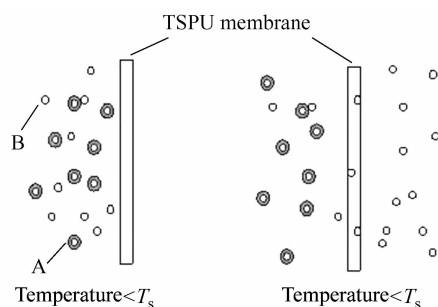
Fig. 12 A possible model for separation of glycine from collagen solution
