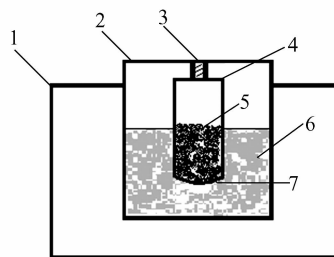
Fig. 2 Apparatus diagram for permeation experiment 1) Oscillator, 2) Flask, 3) Fix setting; 4) A columned cup enclosed with TSPU membrane; 5) Glycine (NaCl, collagen) water solution; 6) The fresh water; 7) The TSPU membrane
