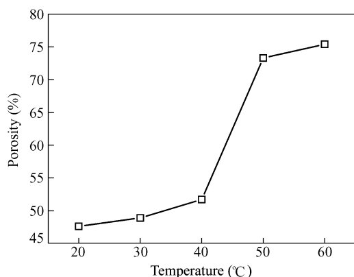
Fig. 9 The porosity of TSPU membrane as a function of temperature
