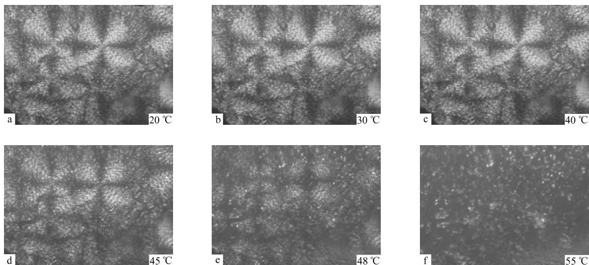
Fig. 5 The POM images of TSPU with crystal soft segment at different temperatures
