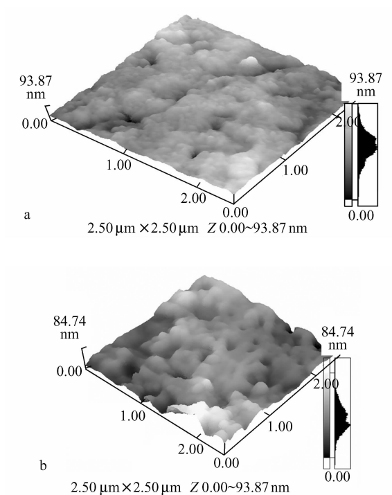
Fig. 7 AFM photographs of the top (a) and bottom surface (b) of TSPU membrane at 20 °C
